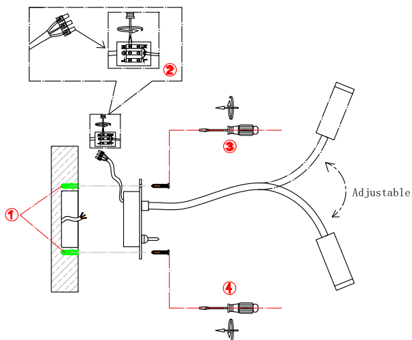
Installation Diagram
